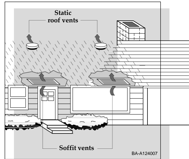
Ventiling helps keep attics cool. Place intake (soffit) vents low and exhaust (static) vents high.
